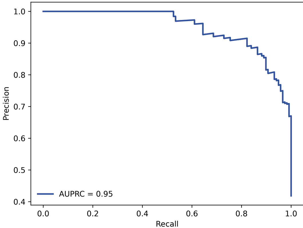
KNN Precision-Recall Curve
